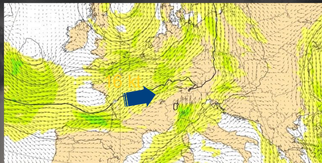
Vents 850 hPa
