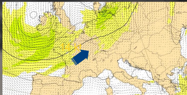
Vents 850 hPa
